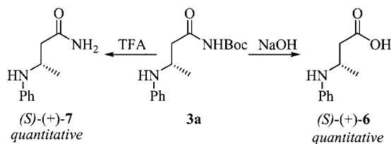
Scheme 3. Conversions to \beta -amino acid and amide
