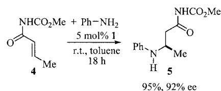
Scheme 2. Conjugate addition of aniline to N -butenoyl-methylcarbamate
