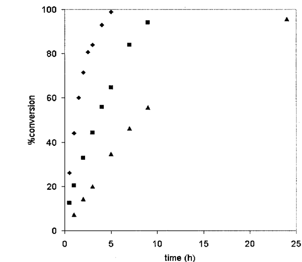
Figure 1. Rate of catalysed addition of p -chloroaniline (diamonds), aniline (squares) and p -anisidine (triangles) to 2a (monitored using 1 H NMR spectroscopy)
