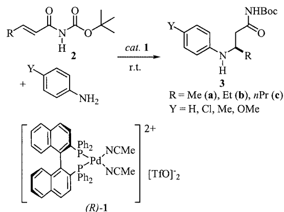
Scheme 1. Conjugate addition of anilines to tert -butyl N -alkenoylcarbamates
